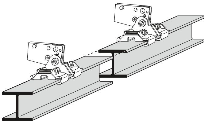
Connestion of steel profiles must not collide with clamps
