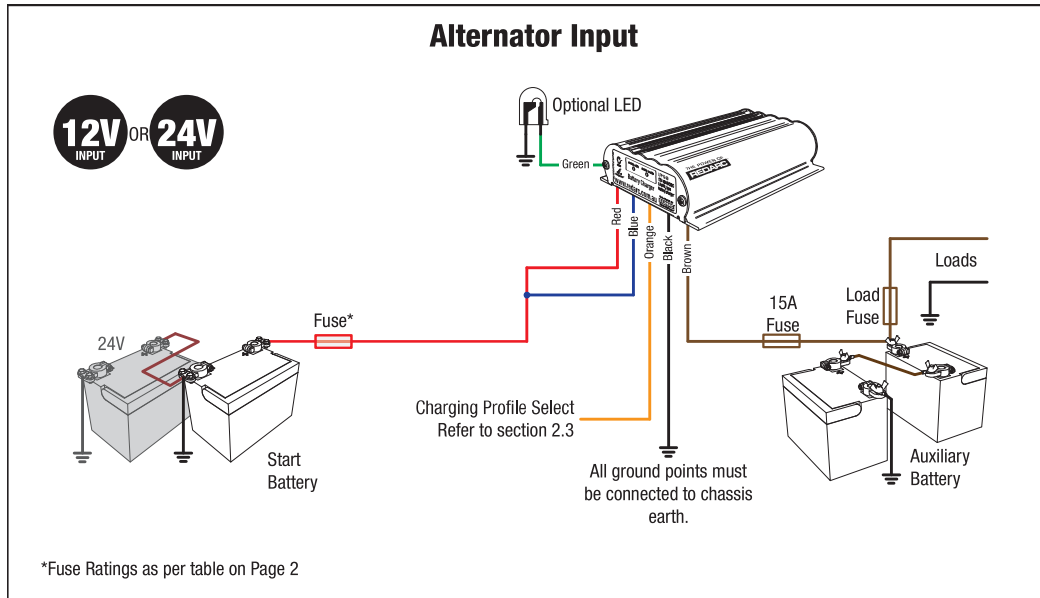
Figure 2.8a - Standard setup for input from a 12V or 24V Start Battery
