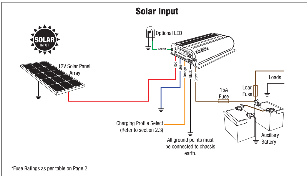
Figure 2.8b - Standard setup for input from a 12V Solar array
