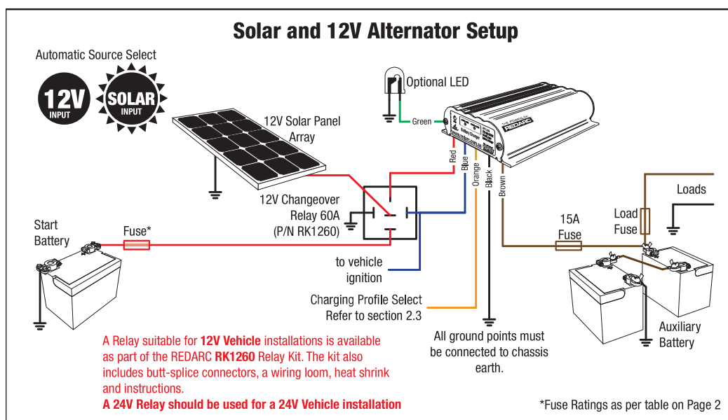
Figure 2.8c - Using a changeover relay for 12V Start Battery & 12V Solar array inputs
