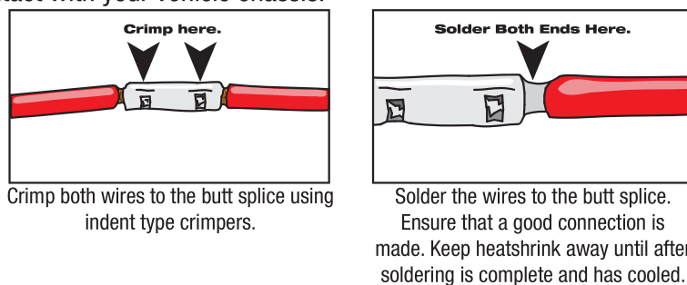
Figure 2.8 - Ensuring a good wiring connection
