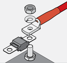
MIDI Fuse Assembly
